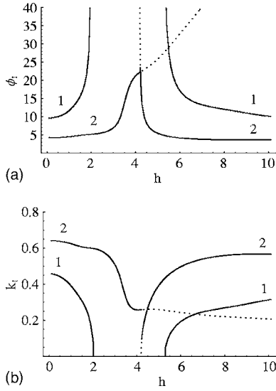
FIG. 7. (a) The critical flow rate of the transverse mode and (b) the wave number. a=30 , \delta=3 , (1) b=12 , and (2) b=7 . The transverse solution always decays in the gap between the curves 1. The dashed parts of the curves 2 indicate solutions that are not, in general, selected by the system.
