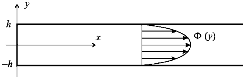
FIG. 1. Sketch of a 2D reactor with parabolic Poiseuille flow.
