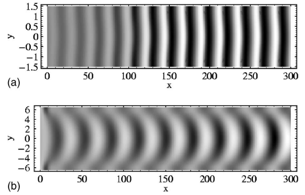
FIG. 2. Transverse steady-state solutions to the system (1)–(3) at a=30 , b=12 , \delta=3 , and \phi=17 . Gray levels are proportional to the values of u : the lighter tone represents higher values. (a) h=1.5 , (b) h=6.5 . U_{\text{bnd}}(y) \equiv 0.5 , V_{\text{bnd}}(y) \equiv 0 .
