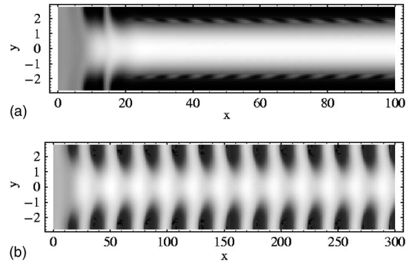
FIG. 5. Transition from the longitudinal solution (a) to the transverse one when the flow rate grows. a=30 , b=12 , \delta=9 , h=2.8 , U_{\text{bnd}}(y)\equiv 0.5 , V_{\text{bnd}}(y)\equiv 0 . (a) \phi=5 , (b) \phi=18 ( \phi_t\approx 16.0 ). The solution in (b) is stationary, while in (a) the toothlike pattern travels in the x direction.
