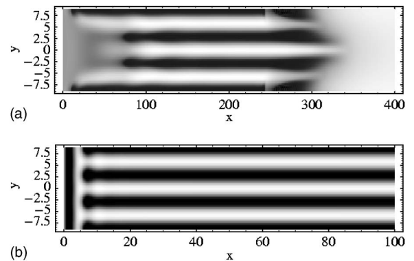
FIG. 3. Longitudinal solutions for n=6 , a=30 , b=12 , \delta=9 , h=9 , U_{\text{bnd}}(y) \equiv 0.5 , V_{\text{bnd}}(y) \equiv 0 . (a) is a snapshot of the formation of the stationary pattern behind the moving arrowed front, \phi=25 . (b) is the steady state for \phi=0 when the structure (a) is taken as the initial state.
