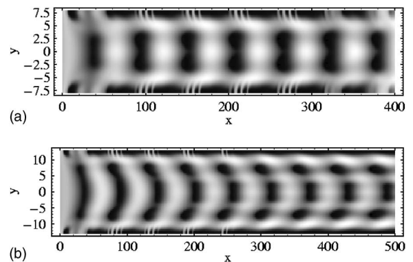
FIG. 6. The stationary spot solution as a composition of the transverse and longitudinal structures. a=30 , b=12 , \delta=7 , \phi=30 , U_{\text{bnd}}(y)\equiv 2 , V_{\text{bnd}}(y)\equiv 0 . (a) h=8 , (b) h=13 .
